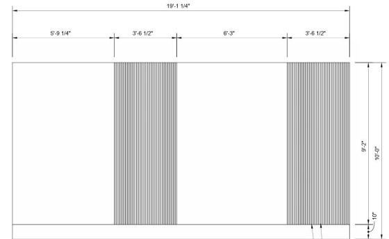
ELEVATION VIEW WALL (B)
